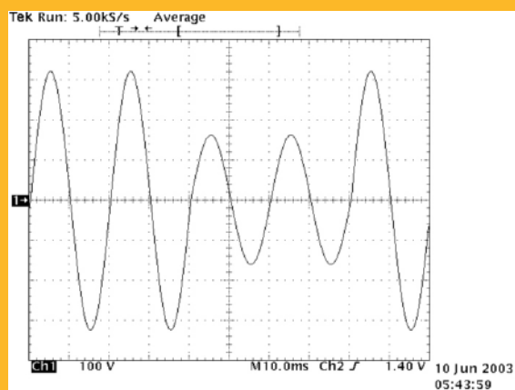
Burst fire waveform
