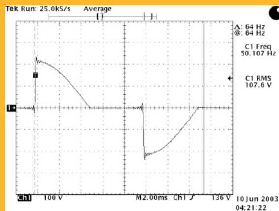
Phase-fired waveform
