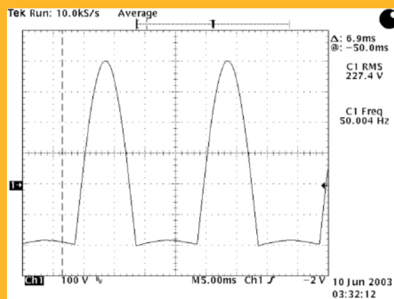
Half-wave rectified waveform
